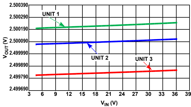
FIGURE 5. LINE REGULATION, THREE UNITS
