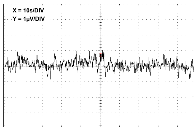
FIGURE 18. V_{OUT} vs NOISE, 0.1Hz to 10Hz
