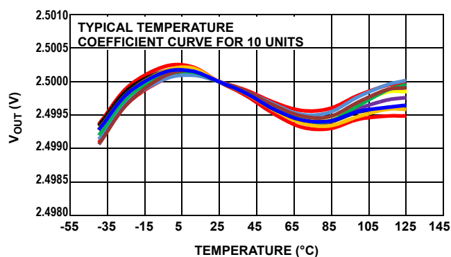
FIGURE 2. V_{\text{OUT}} vs TEMPERATURE
