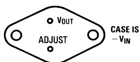
Bottom View Steel TO-3 Metal Can Package (K STEEL) Order Number LM333K STEEL See NS Package Number K02A
