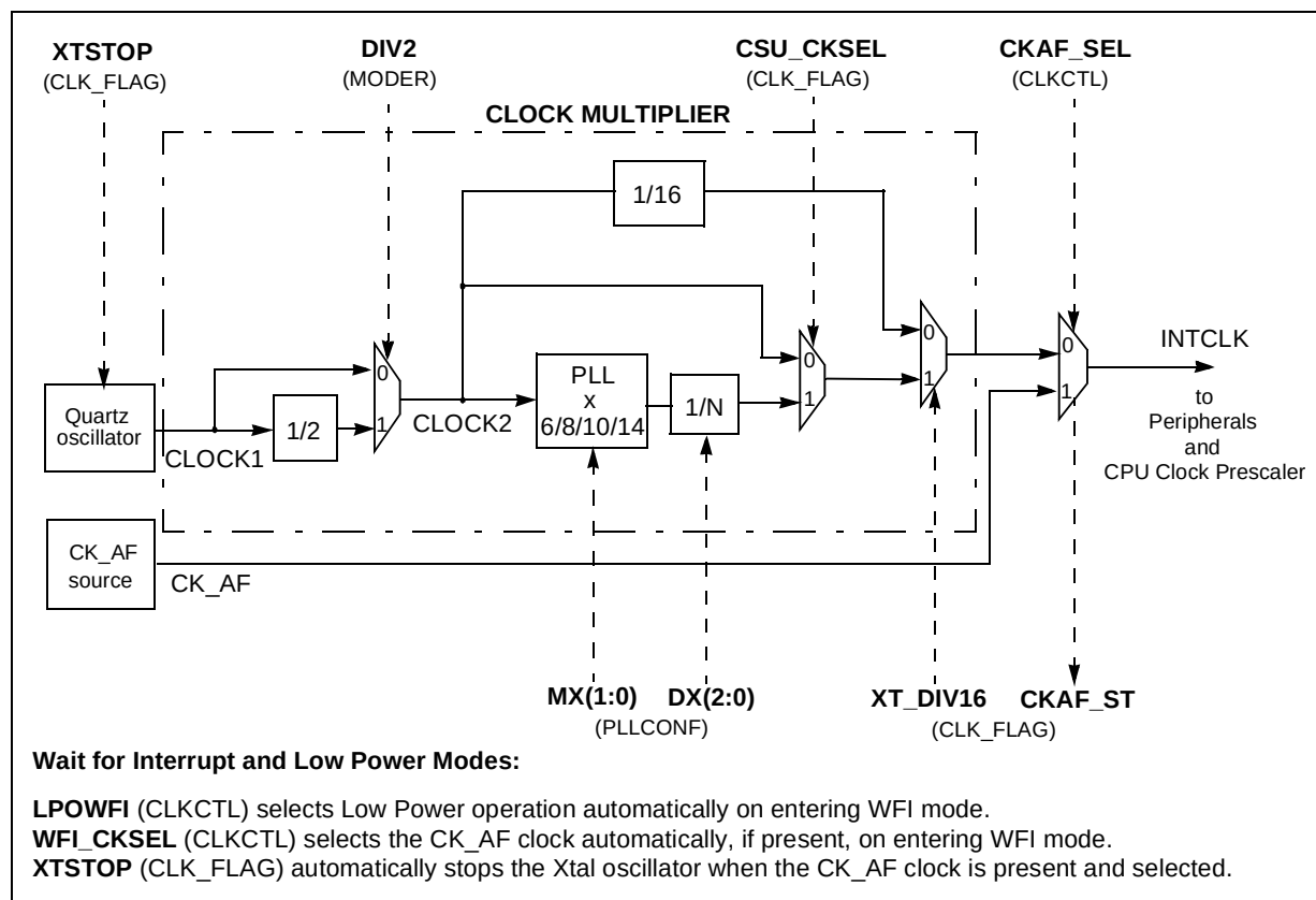
Figure 26. Clock Control Unit Programming
