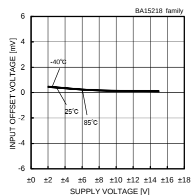
Input Offset Voltage - Supply Voltage (Vicm=0[V], Vout=0[V])
