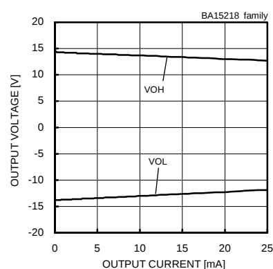
Maximum Output Voltage - Output Current (VCC/VEE=+15[V]/-15[V], Ta=25[°C])
