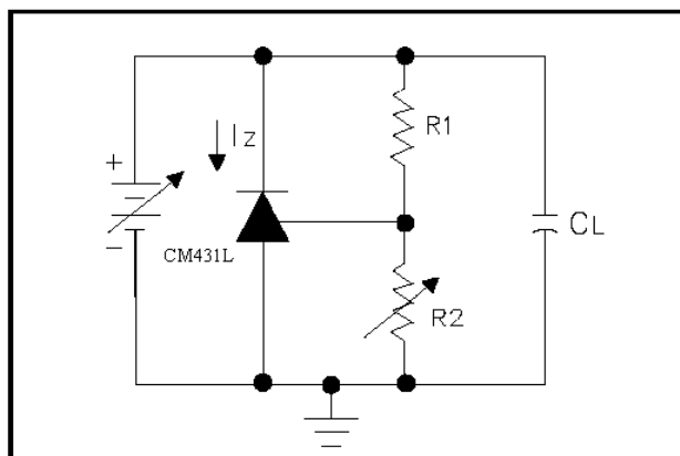
Stability Circuit
