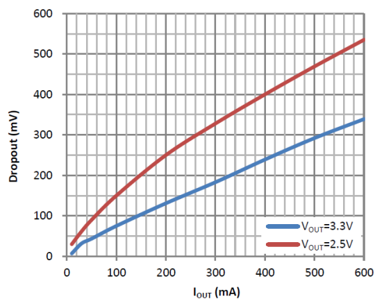
5. Dropout Voltage
