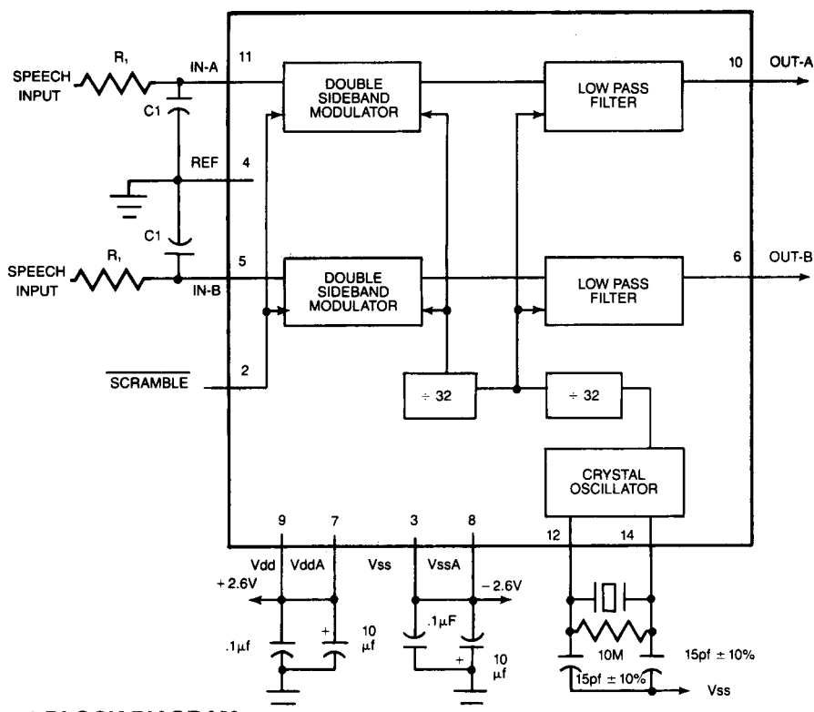
Figure 1 BLOCK DIAGRAM
