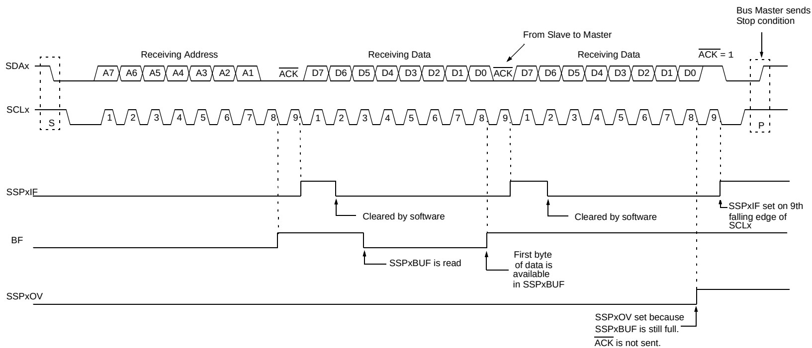
FIGURE 15-14: I 2 C SLAVE, 7-BIT ADDRESS, RECEPTION (SEN = 0, AHEN = 0, DHEN = 0)
