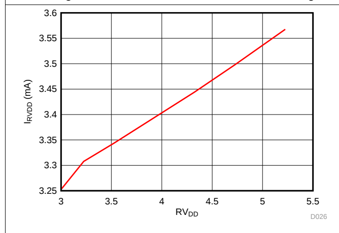
Figure 26. Analog Supply Current vs Supply Voltage
