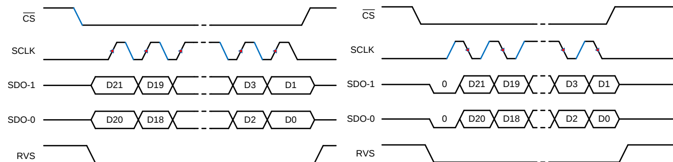
Figure 57. SPI-00-D Protocol
