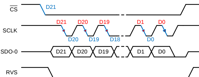
Figure 56. SPI-10-S-EDL Protocol, 22 SCLKs
