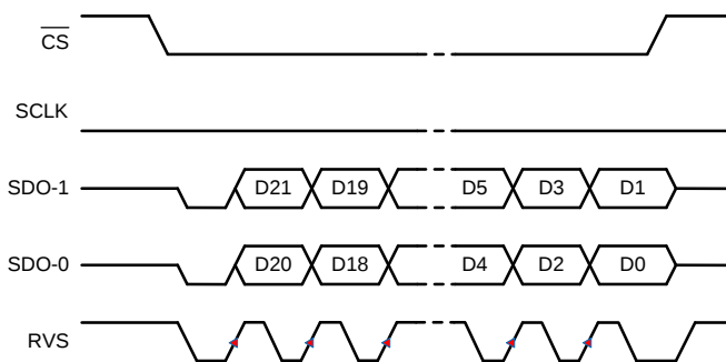
Figure 75. SRC-INT-DS: SRC, INTCLK, Dual SDO, SDR
