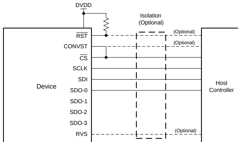
Figure 83. SPI Interface, Minimum Pins
