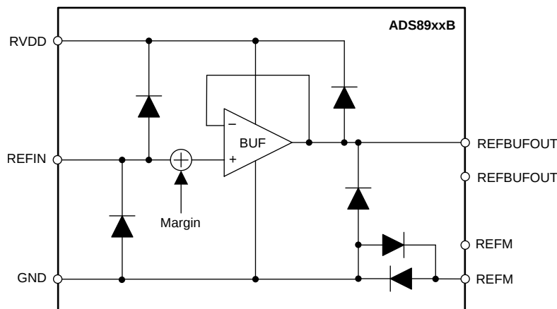
Figure 29. Internal Reference Buffer Block Diagram
