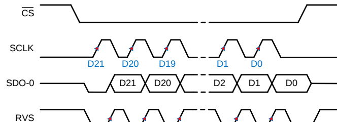
Figure 70. SRC-EXT-SS: SRC, SCLK, Single SDO, SDR
