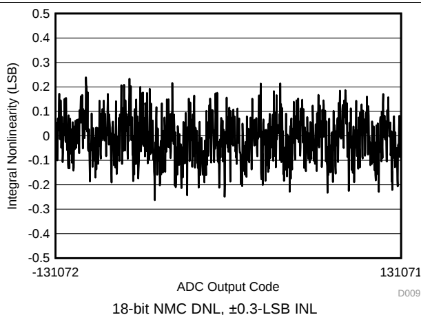
Figure 101. Typical Linearity
