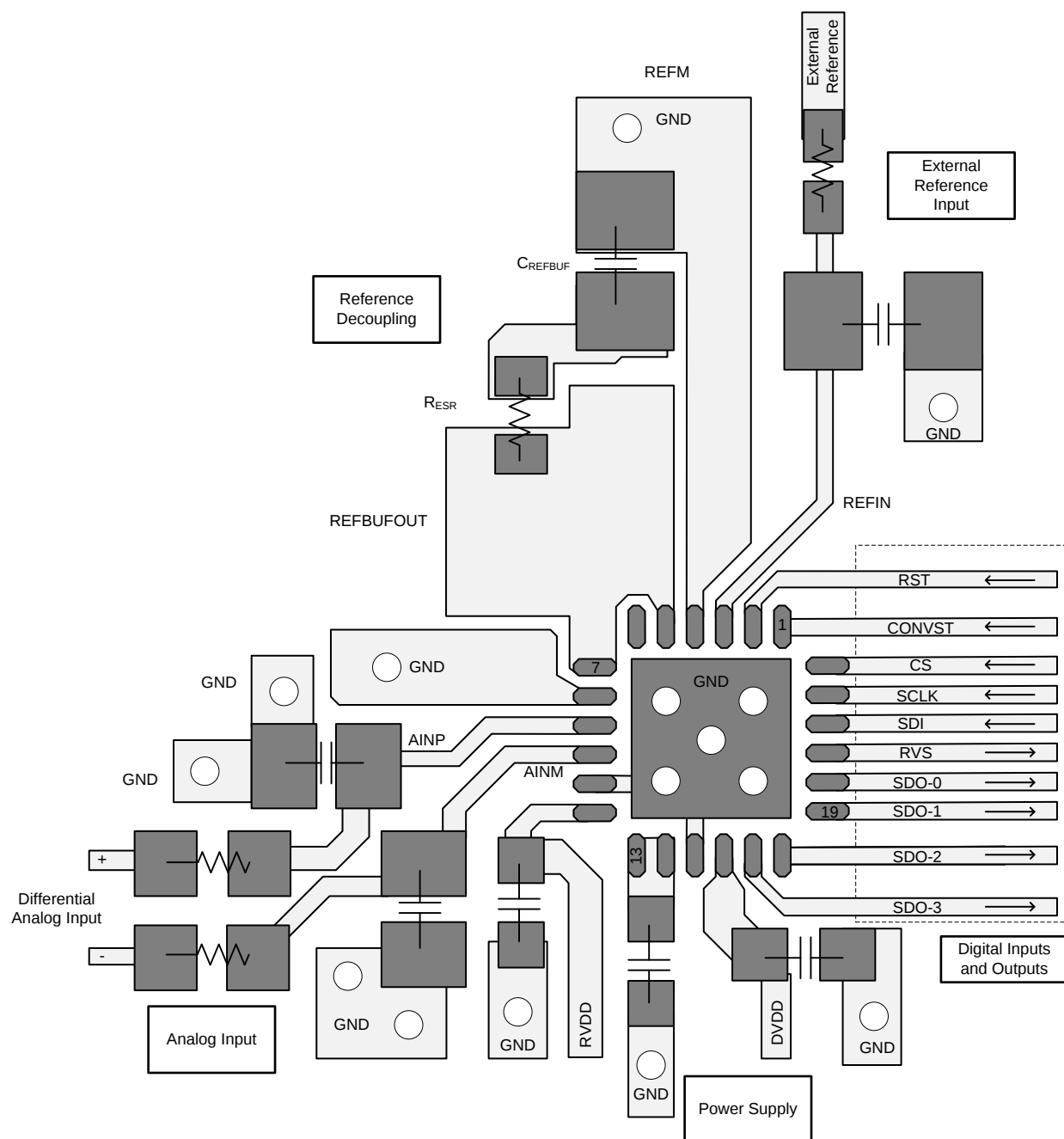
Figure 104. Recommended Layout
