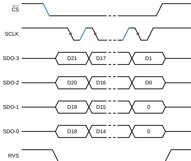
Figure 63. SPI-10-Q Protocol
