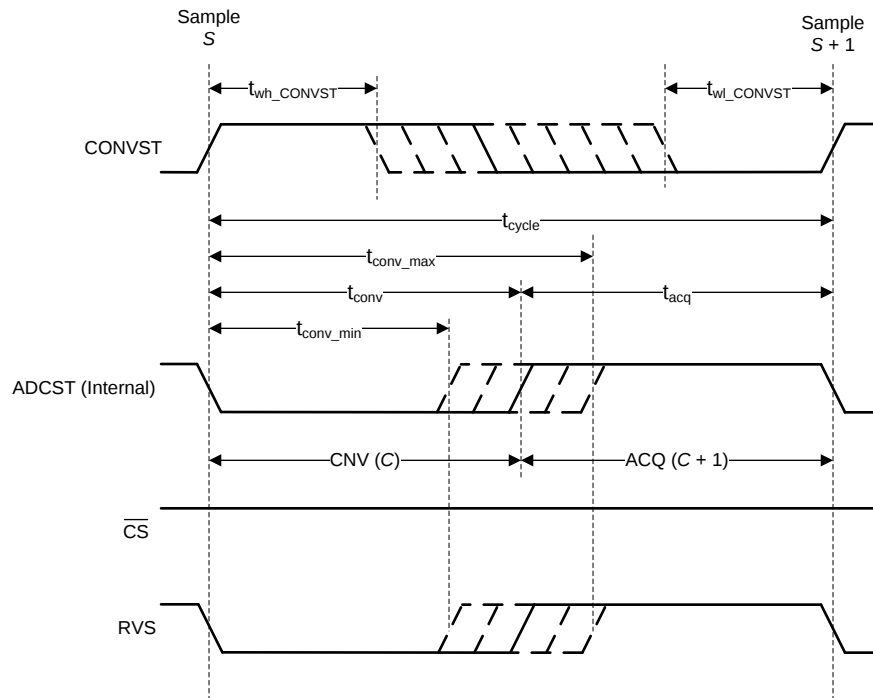
Figure 37. Typical Conversion Process
