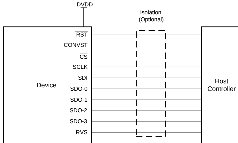
Figure 82. MultiSPI Digital Interface, All Pins
