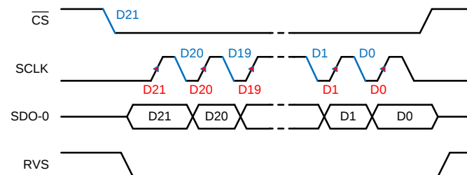
Figure 51. SPI-00-S Protocol, 22 SCLKs
