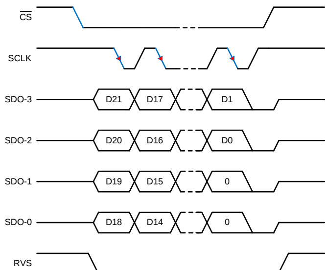
Figure 68. SPI-10-Q-EDL Protocol
