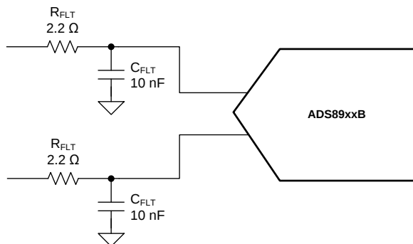
Figure 99. Charge Kickback Filter Configuration
