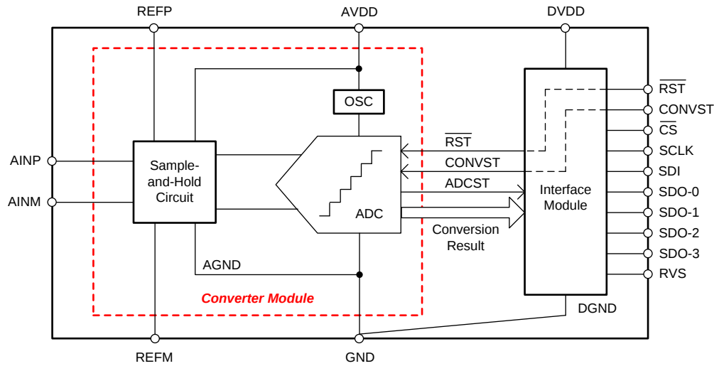
Figure 31. Converter Module
