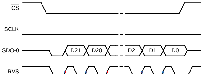
Figure 71. SRC-INT-SS: SRC, INTCLK, Single SDO, SDR
