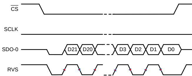
Figure 73. SRC-INT-SD: SRC, INTCLK, Single SDO, DDR
