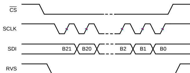
Figure 50. SPI-11-S Protocol, Optimal Command Frame
