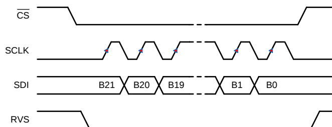
Figure 47. SPI-00-S Protocol, Optimal Command Frame
