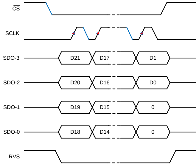
Figure 61. SPI-00-Q Protocol
