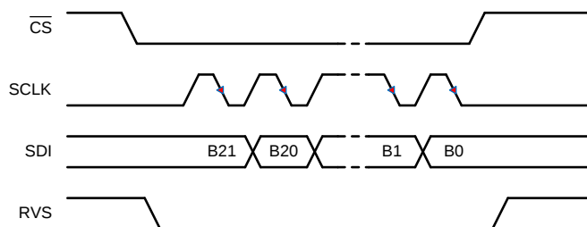
Figure 48. SPI-01-S Protocol, Optimal Command Frame
