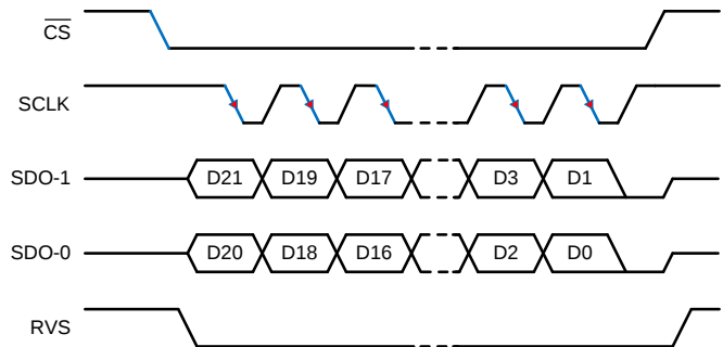
Figure 66. SPI-10-D-EDL Protocol
