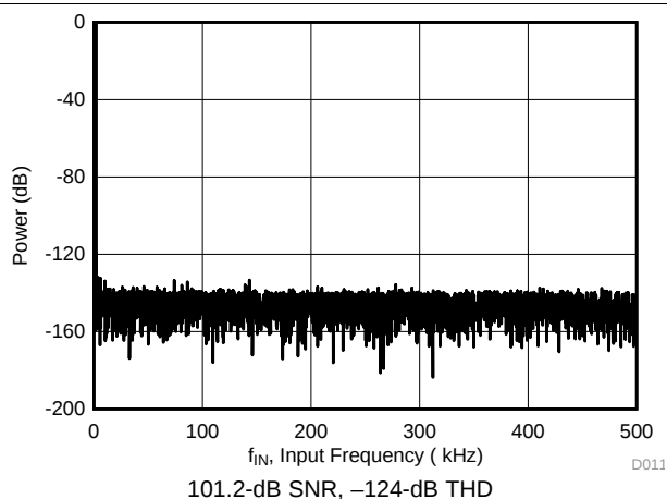
Figure 102. Noise-Performance FFT Plot
