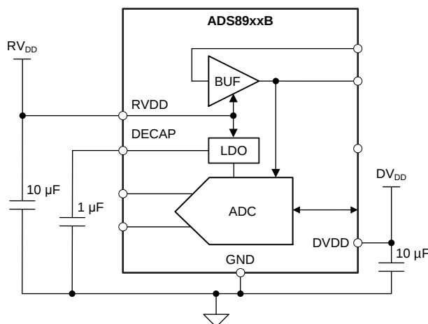
Figure 103. Power-Supply Decoupling
