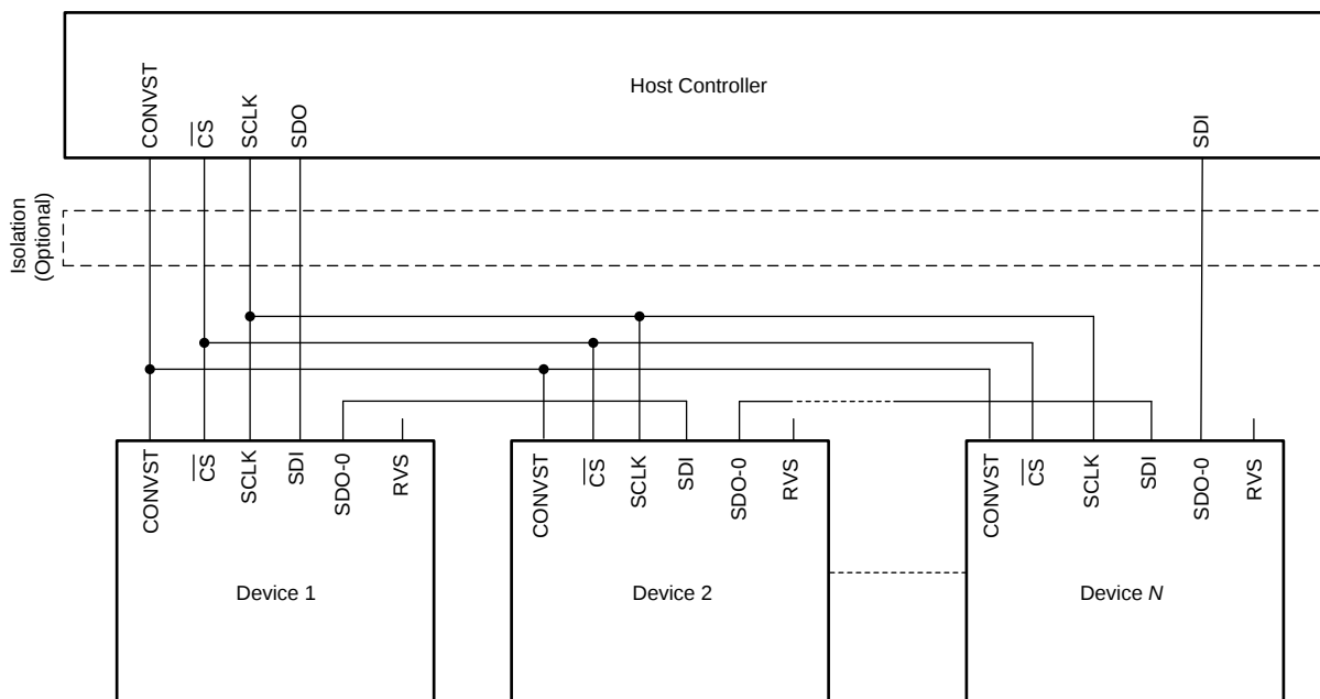
Figure 84. Daisy-Chain Connections
