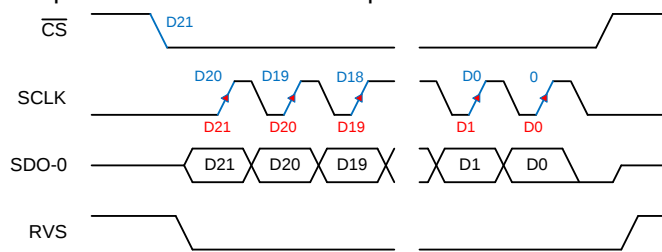
Figure 55. SPI-00-S-EDL Protocol, 22 SCLKs
