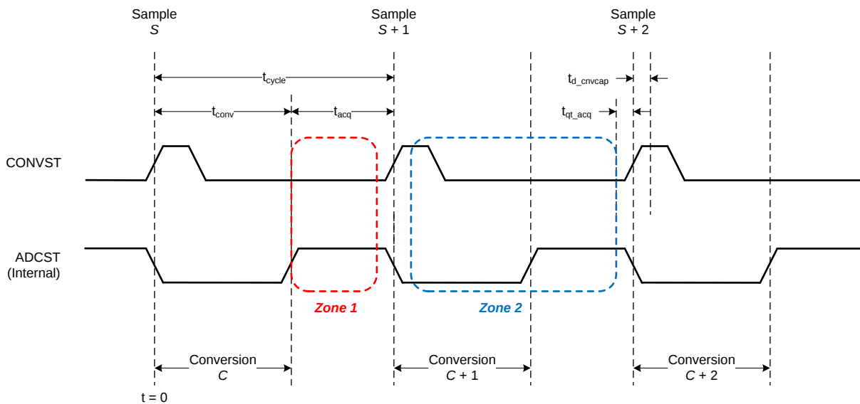
Figure 41. Data Transfer Zones
