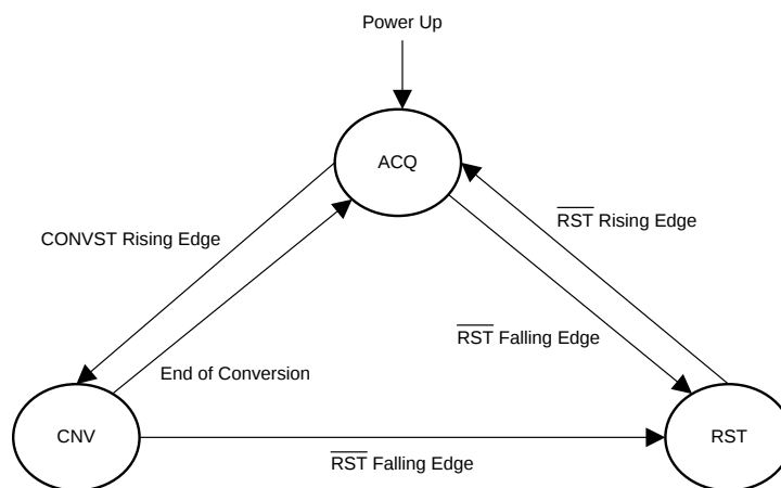
Figure 35. Device Functional States
