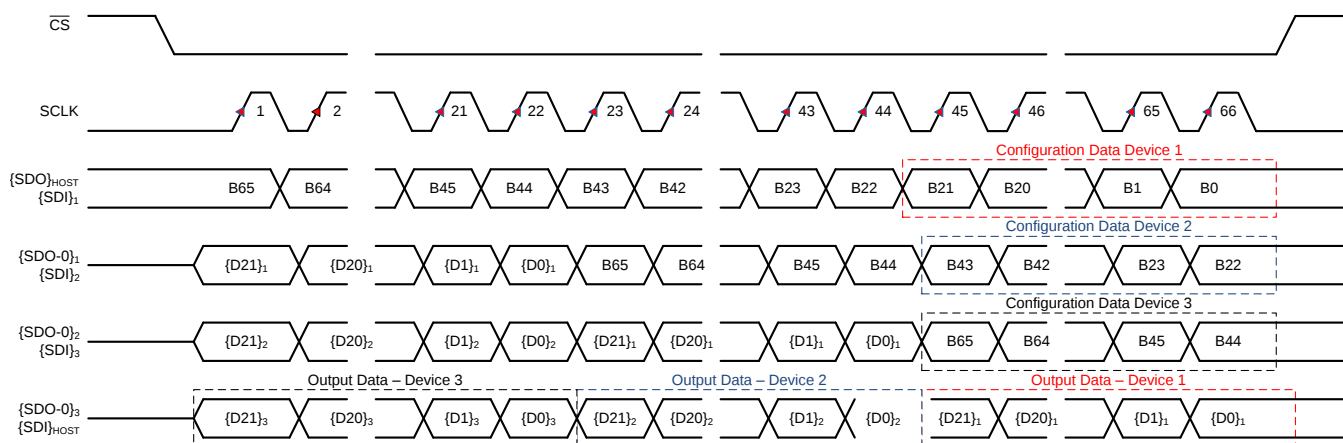
Figure 86. Three-Device, Daisy-Chain Timing
