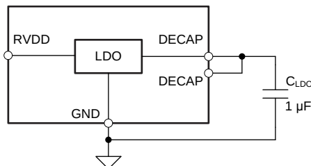
Figure 28. Internal LDO Connections
