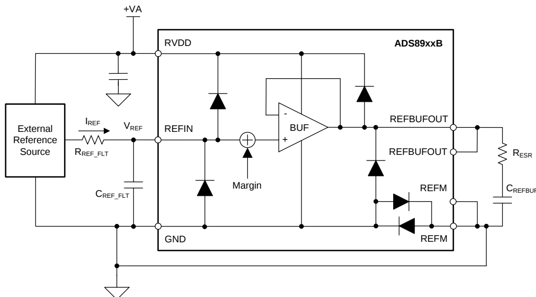
Figure 30. External Connections for the Internal Reference Buffer
