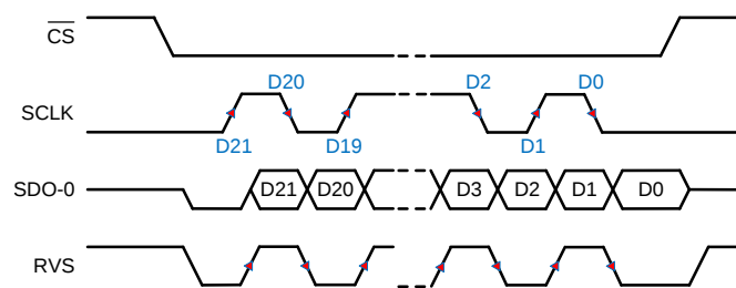
Figure 72. SRC-EXT-SD: SRC, SCLK, Single SDO, DDR
