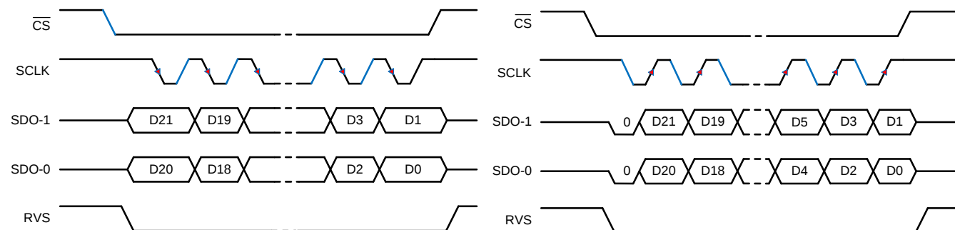
Figure 59. SPI-10-D Protocol
