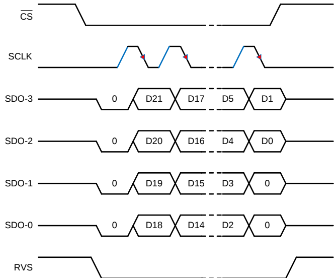
Figure 62. SPI-01-Q Protocol
