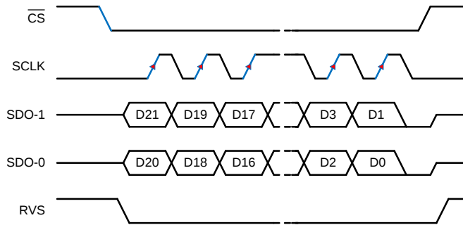
Figure 65. SPI-00-D-EDL Protocol
