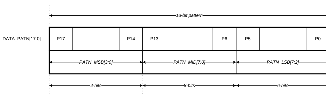
Figure 96. DATA_PATN[17:0]
