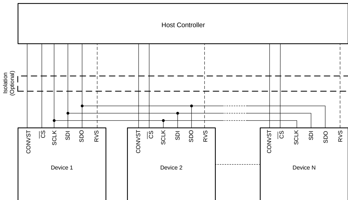
Figure 87. Star-Topology Connection
