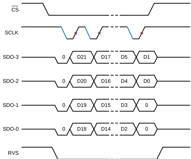
Figure 64. SPI-11-Q Protocol
