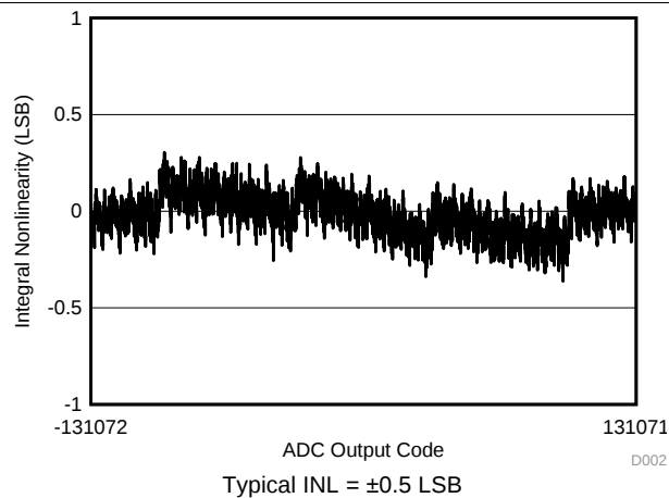
Figure 7. Typical INL
