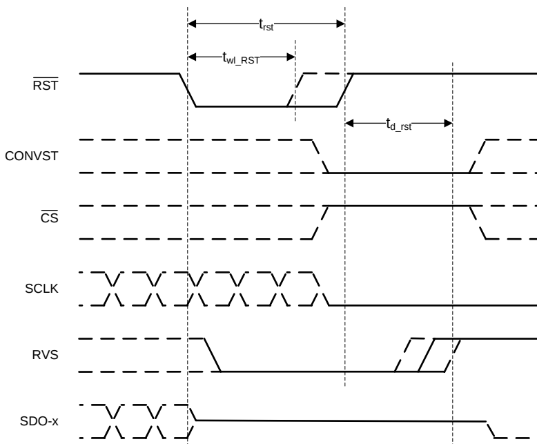
Figure 36. Asynchronous Reset
