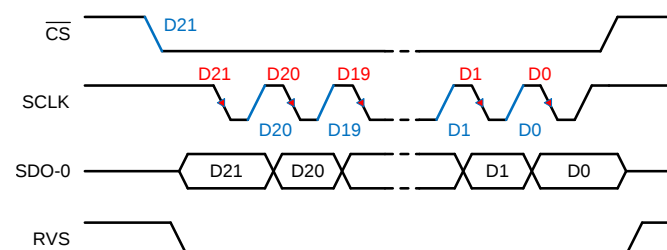
Figure 53. SPI-10-S Protocol, 22 SCLKs
