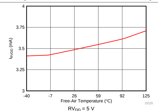
Figure 27. Analog Supply Current vs Temperature
