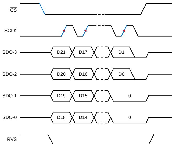
Figure 67. SPI-00-Q-EDL Protocol
