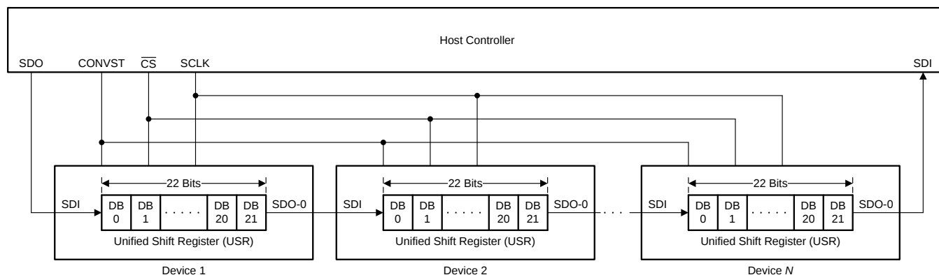
Figure 85. Unified Shift Register
