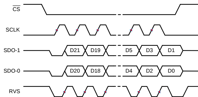
Figure 74. SRC-EXT-DS: SRC, SCLK, Dual SDO, SDR
