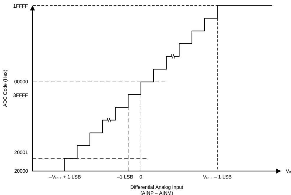
Figure 33. Differential Transfer Characteristics
