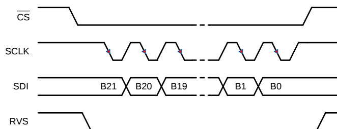
Figure 49. SPI-10-S Protocol, Optimal Command Frame
