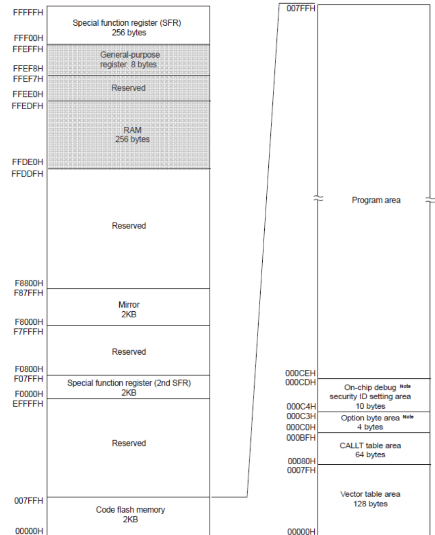
Figure 3-2. Memory Map for the R5F10Y16ASP and R5F10Y46ASP
