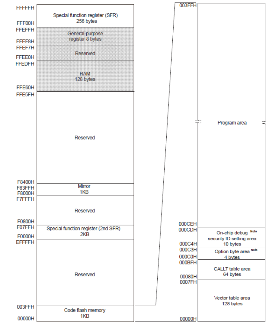
Figure 3-1. Memory Map for the R5F10Y14ASP and R5F10Y44ASP
