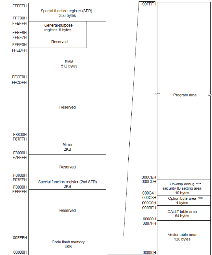
Figure 3-3. Memory Map for the R5F10Y47ASP
