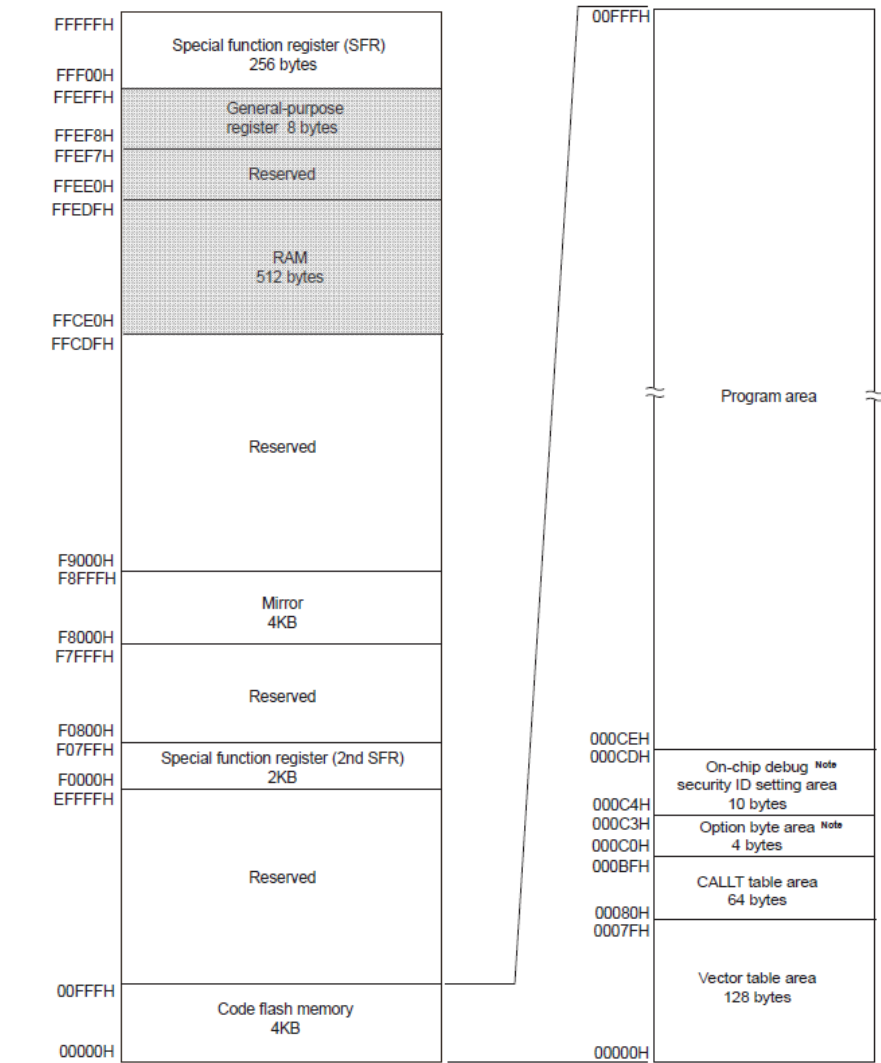
Figure 3-3. Memory Map for the R5F10Y17ASP and R5F10Y47ASP
