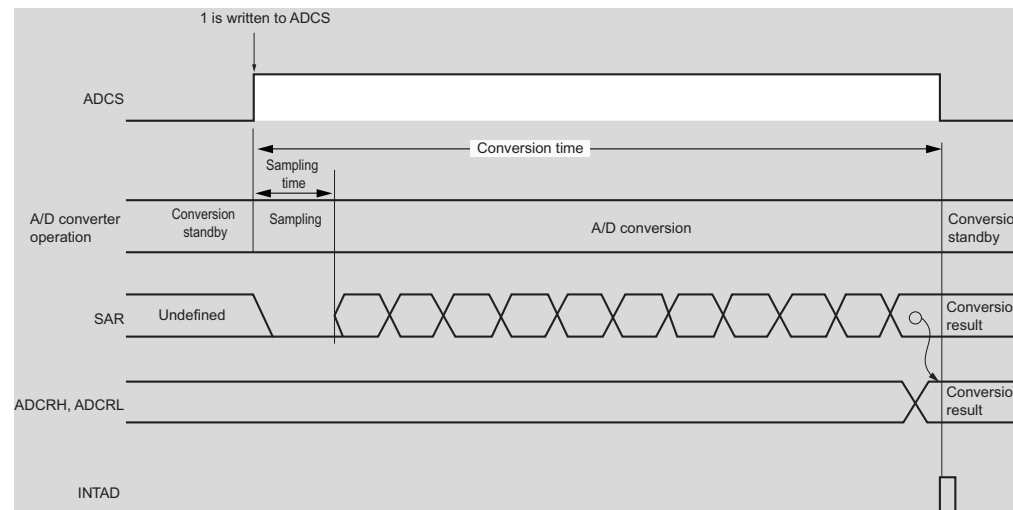
Figure 10-12. Conversion Operation of A/D Converter
