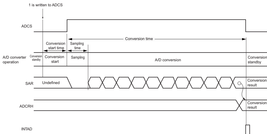
Figure 10-13. Conversion Operation of A/D Converter
