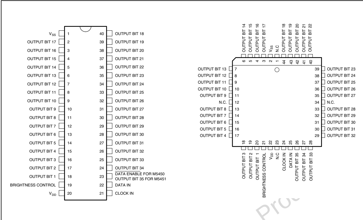
Figure 2. Pin Connection
