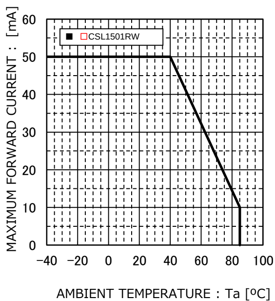
Fig.4 Derating
