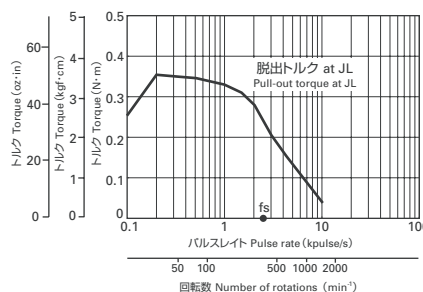
SH1422-5241 (片軸 Single shaft) SH1422-5211 (両軸 Double shafts)
