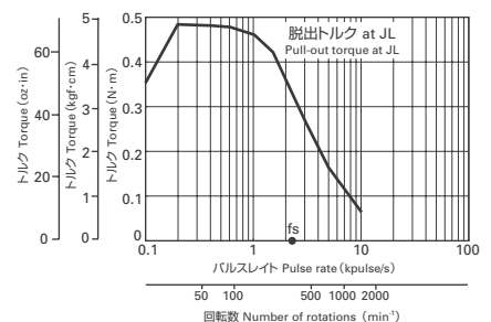
SH1424-5241 (片軸 Single shaft) SH1424-5211 (両軸 Double shafts)
