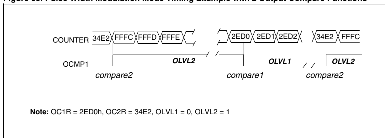
Figure 55. Pulse Width Modulation Mode Timing Example with 2 Output Compare Functions
