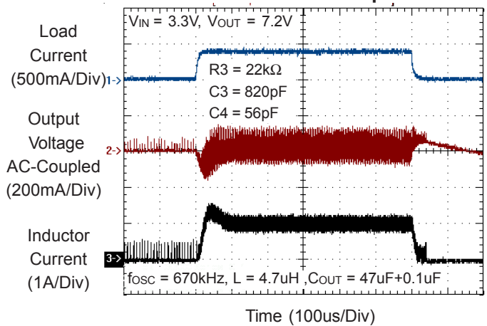
Load-Transient Response
