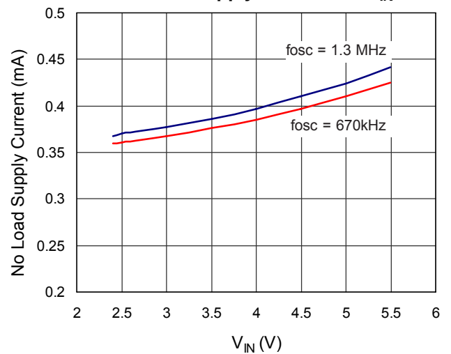
No Load Supply Current vs. V_{IN}
