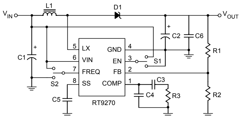
EVB Circuit
