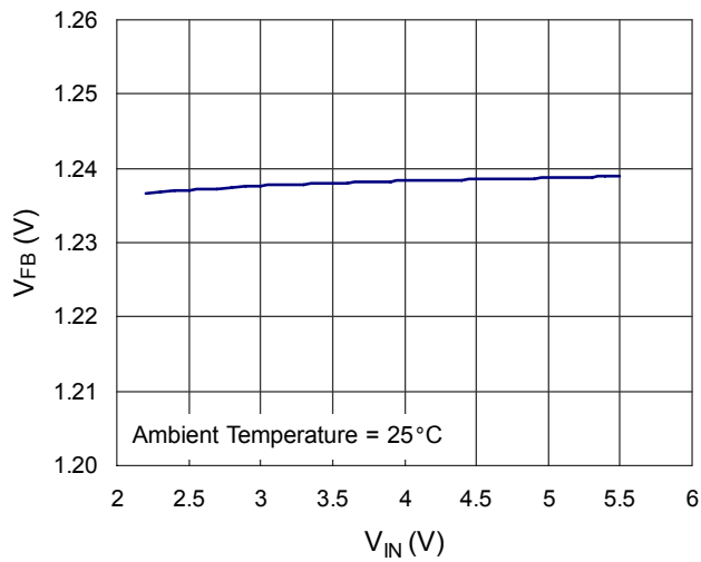
V_{FB} vs. V_{IN}
