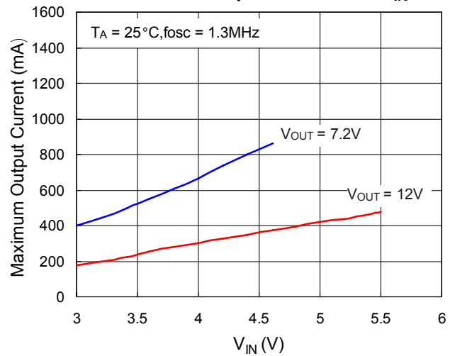
Maximum Output Current vs. V_{IN}
