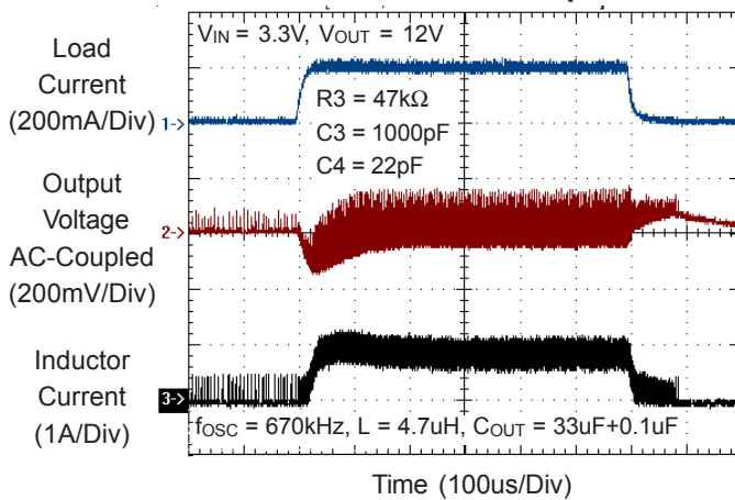
Load-Transient Response
