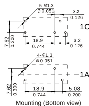
Mounting (Bottom view)
