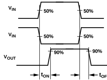
Figure 14. Switching Timing
