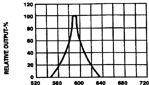
Fig.2 SPECTRAL RESPONSE
