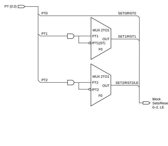
Figure 5. Set/Reset Generator
