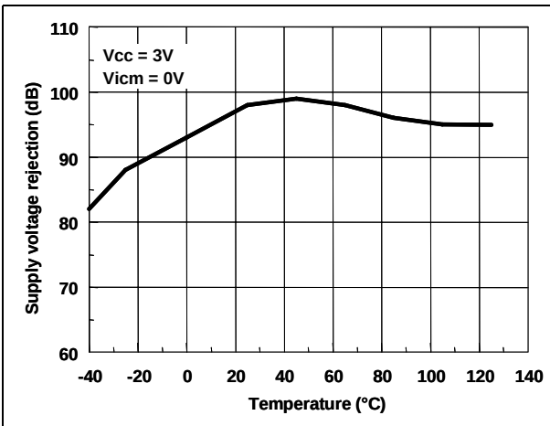
Figure 9. Supply voltage rejection vs. temperature
