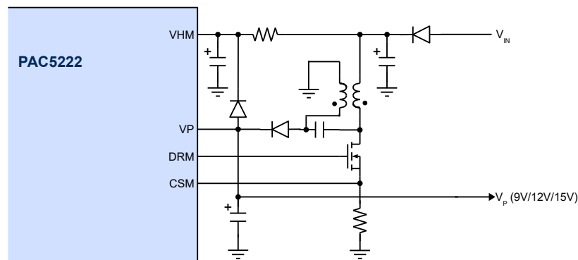
Figure 10-3. SEPIC Mode
