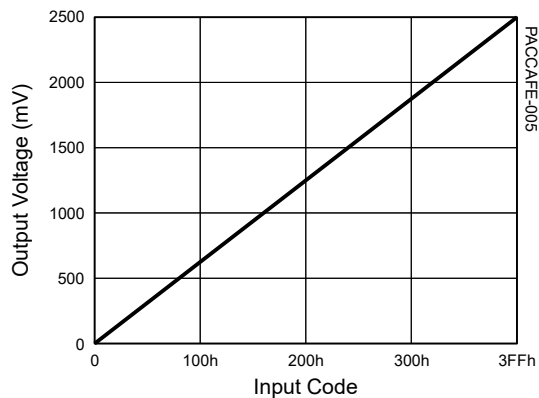
LP DAC Output Voltage vs. Input Code
