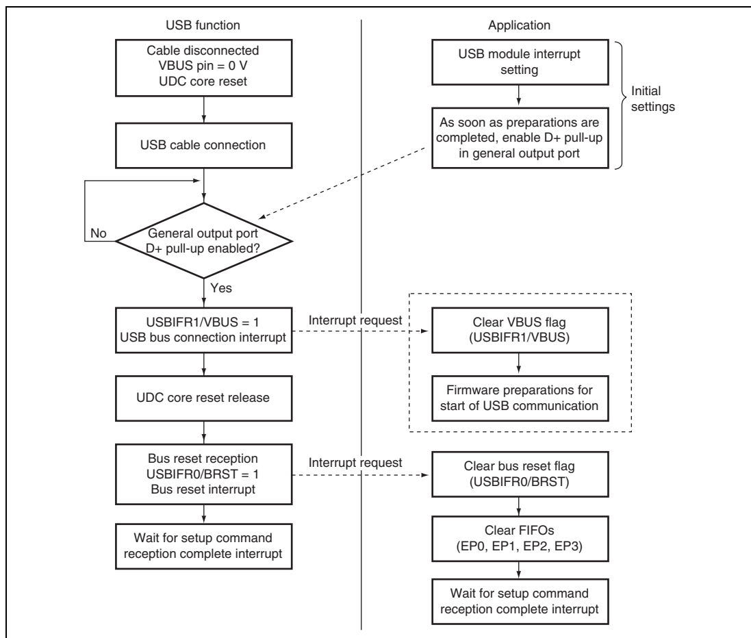
Figure 25.3 Cable Connection Operation
