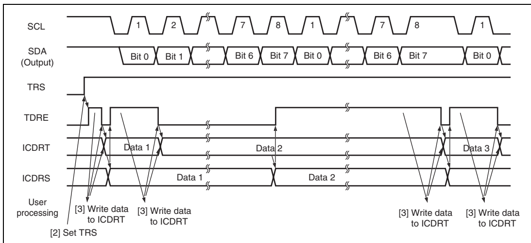
Figure 19.14 Transmit Mode Operation Timing
