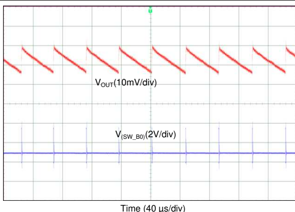
Figure 78. Output Voltage Ripple, PFM Mode (3-Phase Output)
