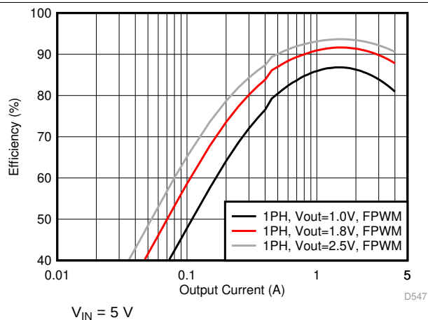
Figure 45. Efficiency in Forced-PWM Mode (1-Phase Output)
