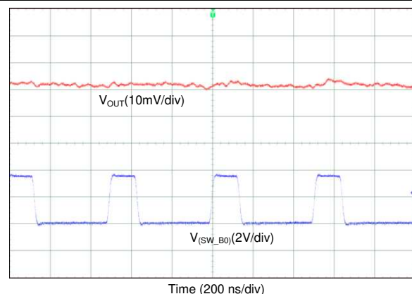
Figure 81. Output Voltage Ripple, Forced-PWM Mode (4-Phase Output)
