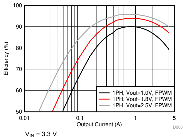
Figure 41. Efficiency in Forced-PWM Mode (1-Phase Output)
