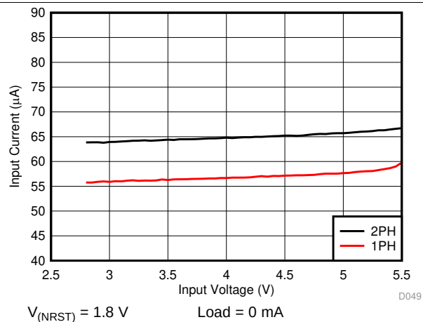
Figure 6. PFM Mode Current Consumption vs Input Voltage, One Regulator Enabled (2+1+1-Phase Output)
