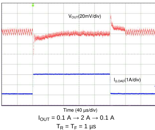
Figure 102. Transient Load Step Response, AUTO Mode (1-Phase Output)
