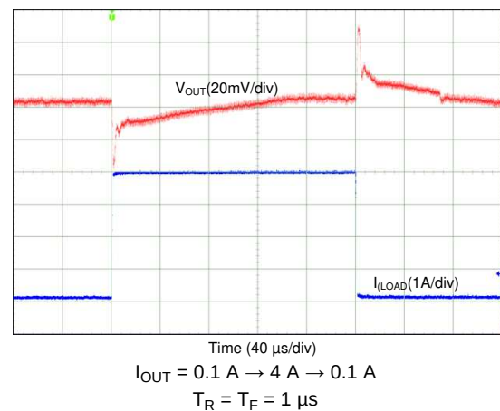
Figure 105. Transient Load Step Response, Forced-PWM Mode (2-Phase Output)
