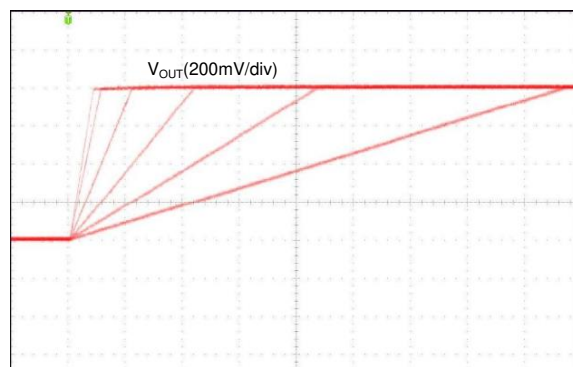
Figure 107. Output Voltage Transition from 0.6 V to 1.4 V With Different Slew Rate Settings
