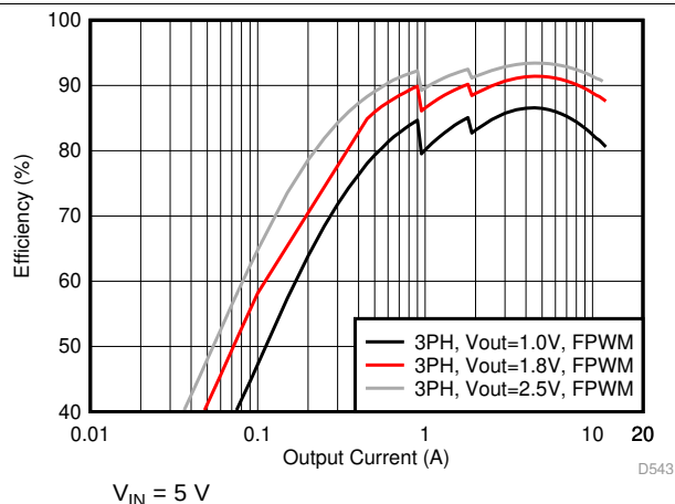
Figure 43. Efficiency in Forced-PWM Mode (3-Phase Output)
