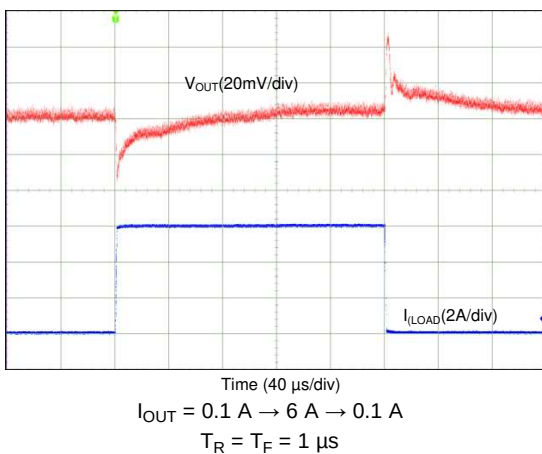
Figure 104. Transient Load Step Response, Forced-PWM Mode (3-Phase Output)
