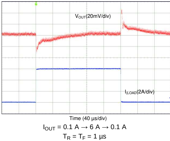
Figure 100. Transient Load Step Response, AUTO Mode (3-Phase Output)
