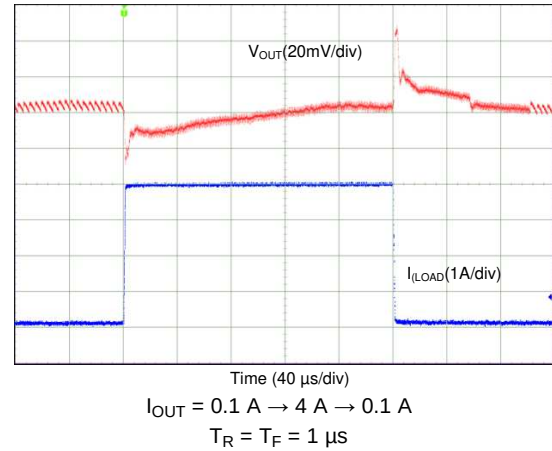
Figure 101. Transient Load Step Response, AUTO Mode (2-Phase Output)
