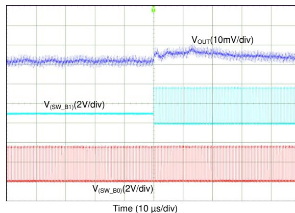
Figure 95. Transient from 1-Phase to 2-Phase Operation (2-Phase Output)
