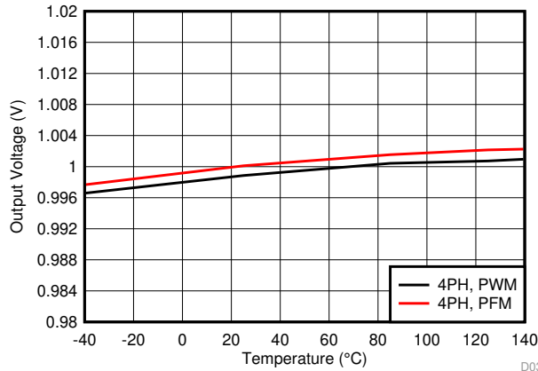
Figure 58. Output Voltage vs Temperature (4-Phase Output)
