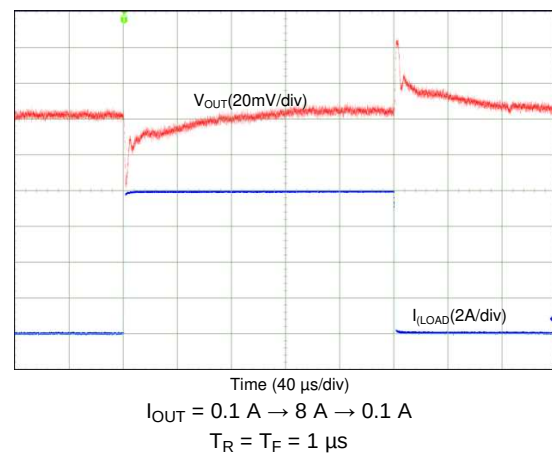
Figure 103. Transient Load Step Response, Forced-PWM Mode (4-Phase Output)
