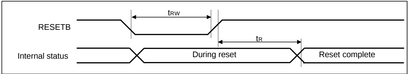
Figure 42. Reset Input Timing
