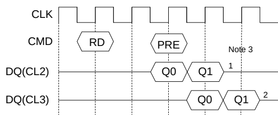
3) Read Interrupted by Precharge (BL=4)
