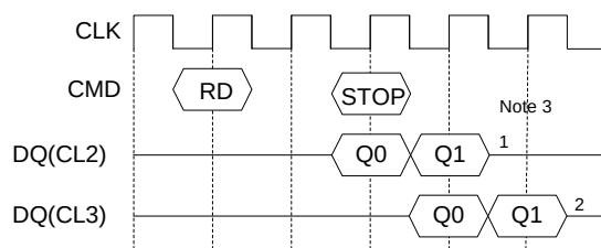
4) Read Burst Stop (BL=4)
