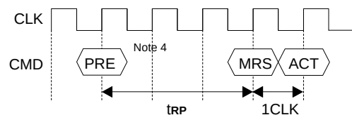
Mode Register Set
