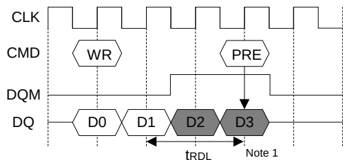
1) Write Interrupted by Precharge (BL=4)
