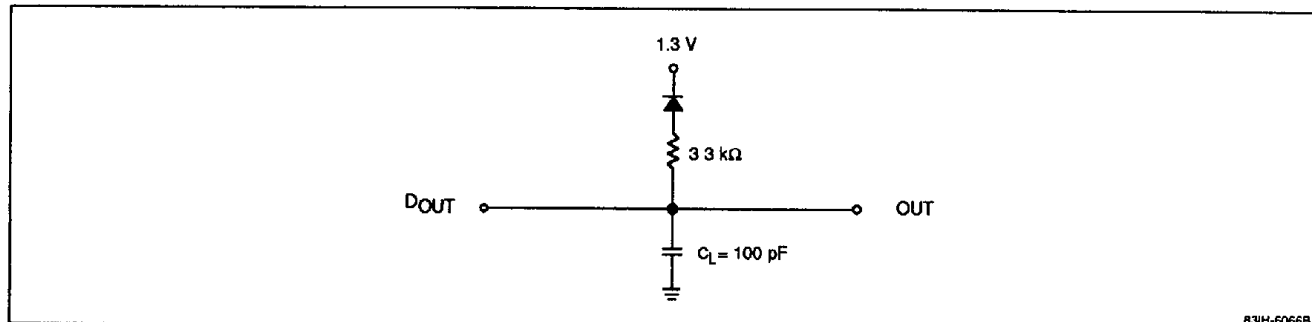
Figure 1. Output Load
