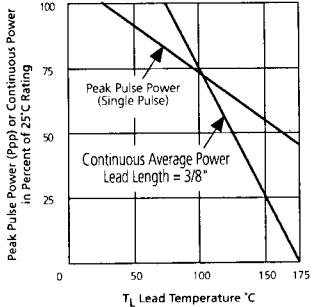
FIGURE 1 Derating Curve
