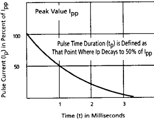
FIGURE 2 Pulse Waveform For Exponential Surge
