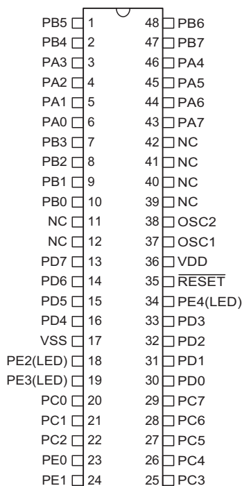
HT82K68E-L/HT82K68A-L —48 SSOP-A
