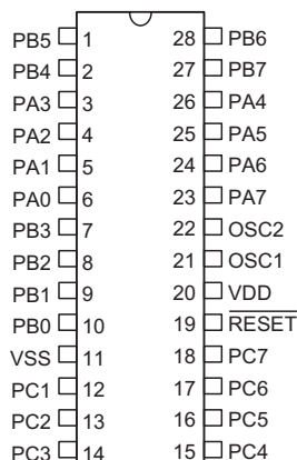
HT82K68E-L/HT82K68A-L —28 SOP-A
