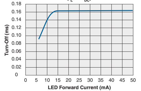
Typical Turn-Off vs. LED Forward Current ( I_L=1A_{DC} )
