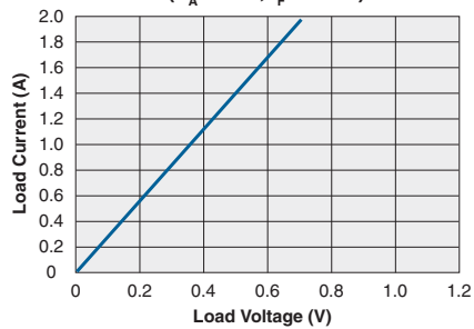
Typical Load Current vs. Load Voltage ( T_A = 25^\circ C , I_F = 10mA )
