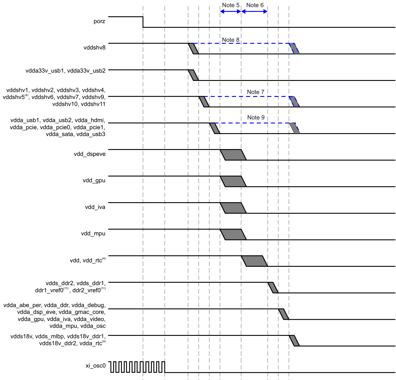
Figure 5-5. Power-Down Sequencing (10)(12)
