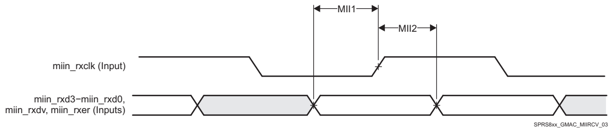
Figure 5-69. GMAC Receive Interface Timing MII operation
