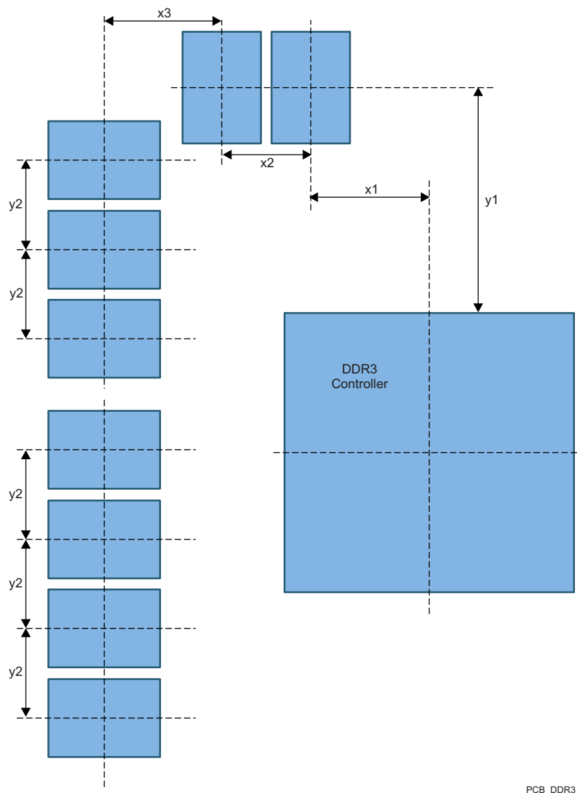
Figure 7-4. Placement Specifications
