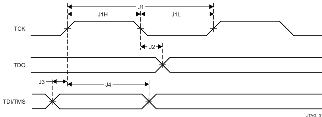
Figure 5-128. JTAG Timing
