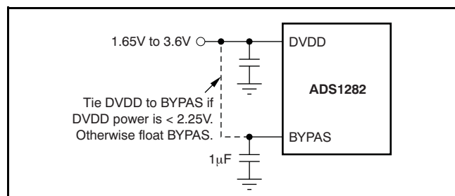
Figure 52. DVDD Power
