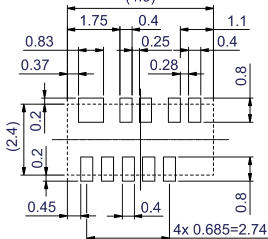
Proposed PCB Footprint (4.9)
