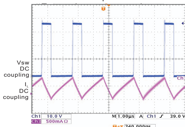
Stable Operation
