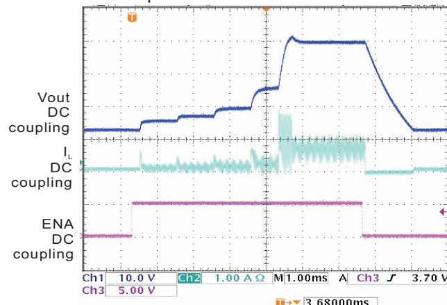
Start up and Shutdown Waveforms
