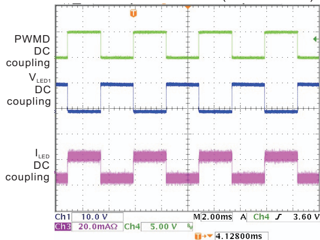
LED Current Waveforms (PWMD=50%)
