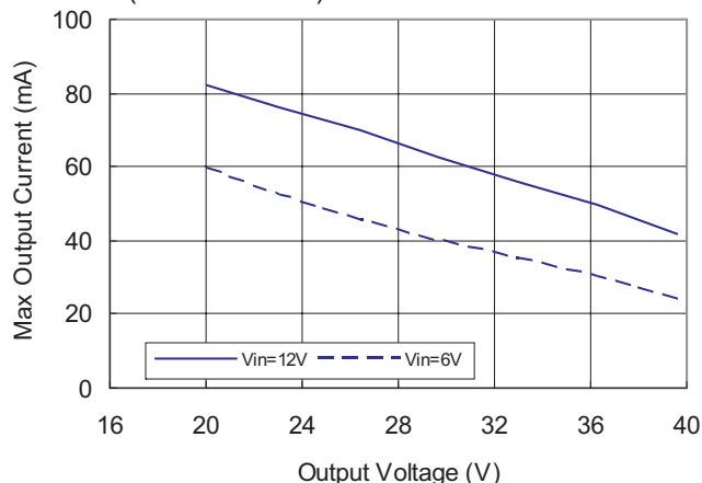
Max Output Current Vs Output Voltage (Per Channel)
