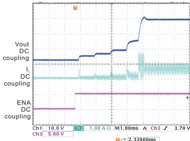
Startup Waveforms
