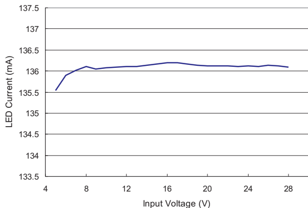
Total LED Current Line regulation
