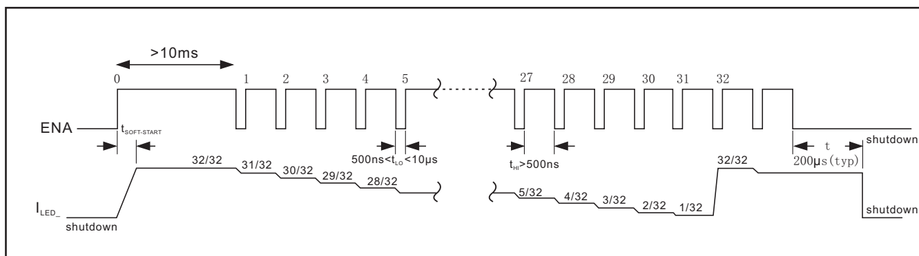
Figure 1. Timing diagram for ENA
