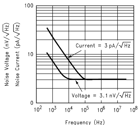
Equivalent Input Noise
