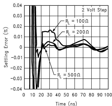
Settling Time vs R_L
