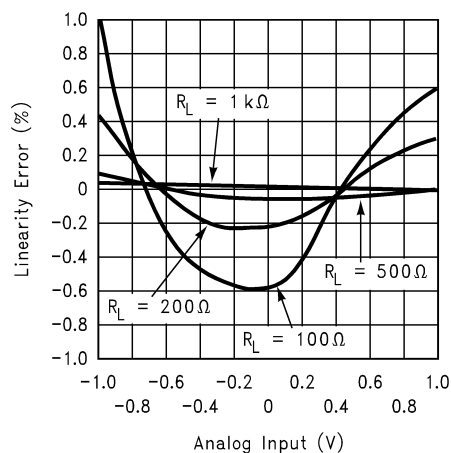
Integral Linearity Error
