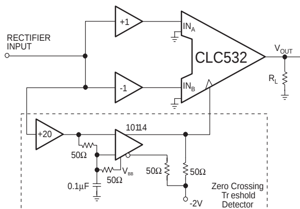
FIGURE 9. Low Distortion Full Wave Rectifier
