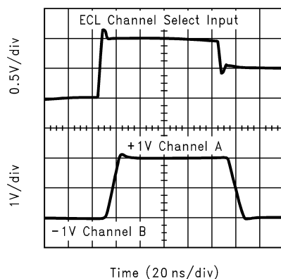
Large signal Channel-to-Channel Switching
