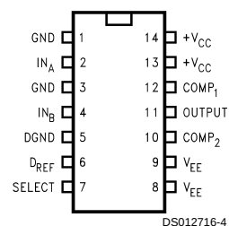
Pinout DIP & SOIC
