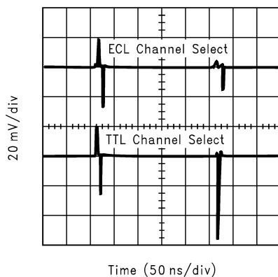
Switching Transient (Grounded Inputs)
