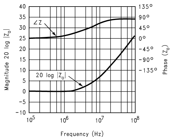
Output Impedance
