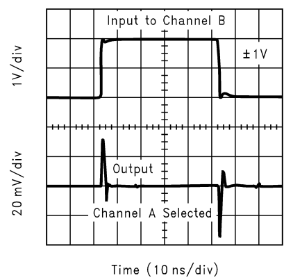
Transient Isolation
