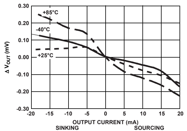
FIGURE 11. LOAD REGULATION
