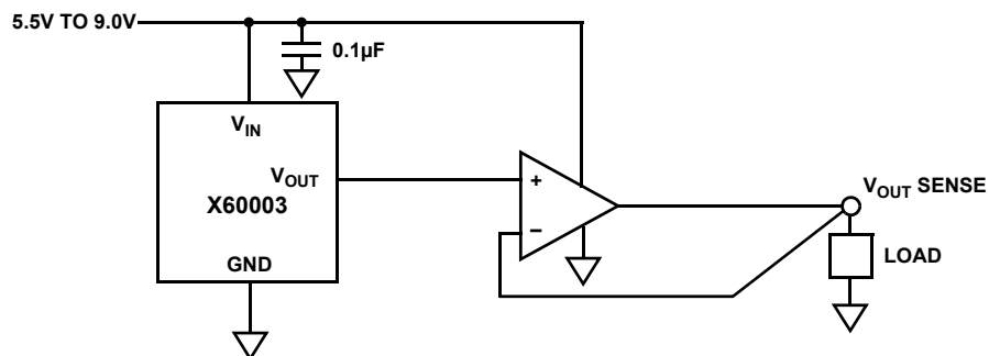
FIGURE 38. KELVIN SENSED LOAD
