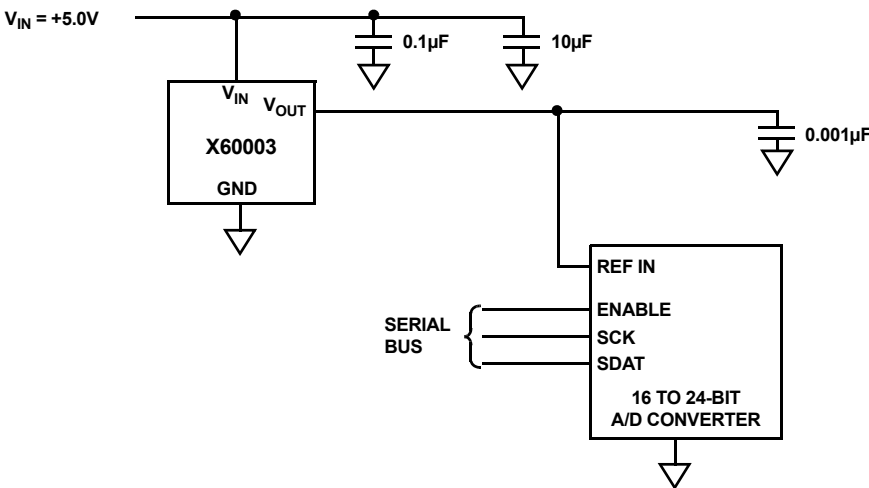
FIGURE 2. TYPICAL APPLICATION PRECISION 16 TO 24-BIT A/D CONVERTER
