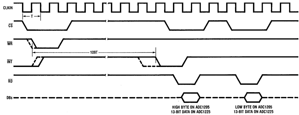
FIGURE 3. Timing Diagram
