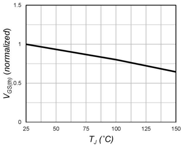
Fig.9 V_{GS(th)} Variation with Temperature (Nomalized)
