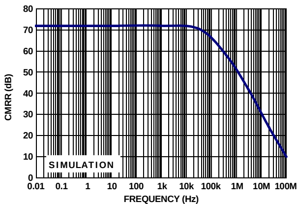
FIGURE 5. CMRR vs FREQUENCY (SIMULATED DATA)
