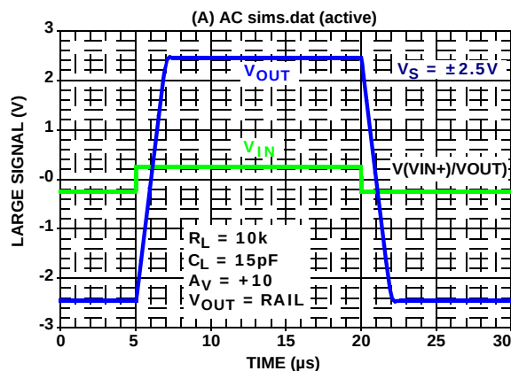
FIGURE 27. SIMULATED LARGE SIGNAL TRANSIENT RESPONSE vs R_L , V_S = \pm 0.9V, \pm 2.5V
