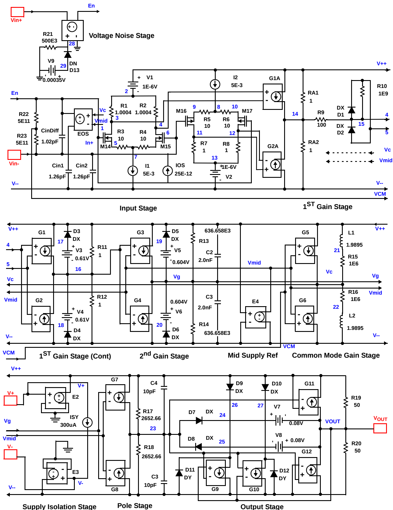
FIGURE 20. SPICE SCHEMATIC
