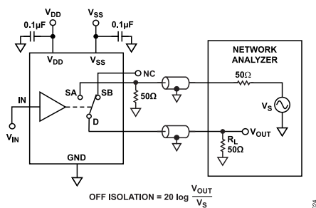
Figure 25. Off Isolation
