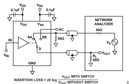
Figure 27. Bandwidth
