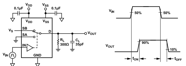
Figure 21. Switching Times, t_{ON} and t_{OFF} ( V_{OUT} is the Output Voltage.)
