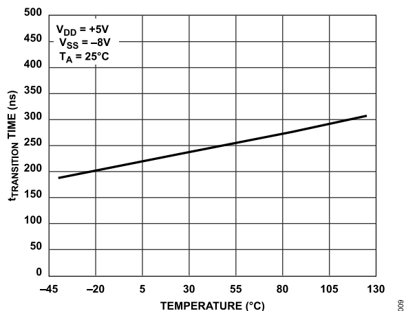
Figure 10. t_{TRANSITION} Time vs. Temperature
