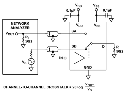
Figure 26. Channel-to-Channel Crosstalk
