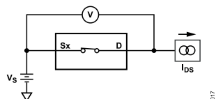
Figure 18. On Resistance ( I_{DS} is the Drain to Source Current.)
