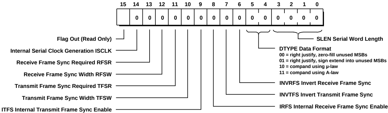
SPORT1 Control Register 0x3FF2
