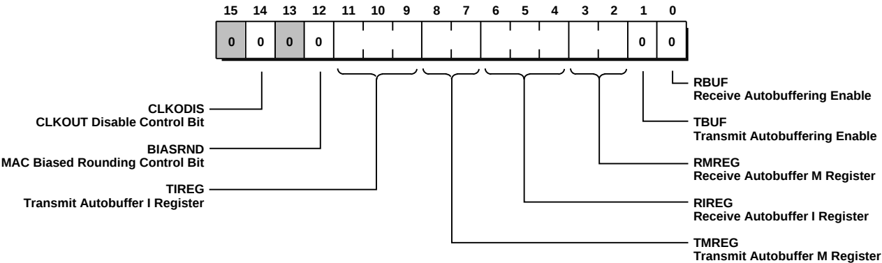
SPORT0 Autobuffer Control Register 0x3FF3
