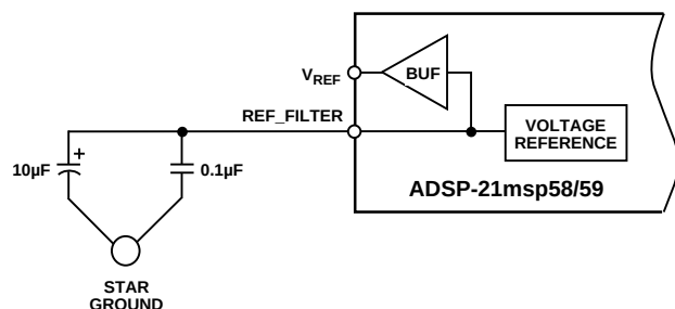
Figure 13. Voltage Reference Filter Capacitor
