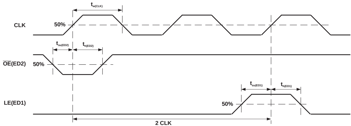
Figure 8. Switching to Special Mode Timing Waveforms
