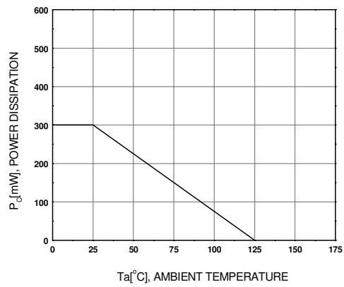
Figure 9. Power Derating
