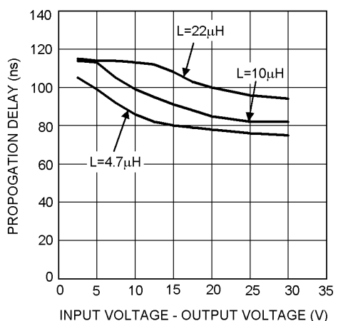
FIGURE 2. Propagation Delay
