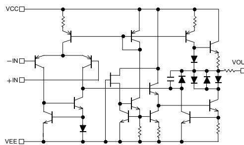
Fig. 225 Simplified schematic (BA14741)
