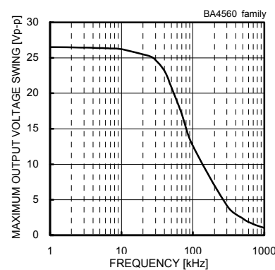
Maximum Output Voltage Swing – Frequency ( V_{CC}/V_{EE}=+15[V]/-15[V] , R_L=2[k\Omega] , T_a=25[^\circ C] )
