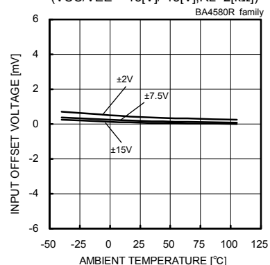
Fig. 98 Input Offset Voltage – Ambient Temperature (Vcm=0[V], Vout=0[V])
