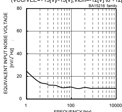
Fig. 129 Equivalent Input Noise Voltage – Frequency ( V_{CC}/V_{EE}=+15[V]/-15[V] , R_s=100[\Omega] , T_a=25[^\circ C] )
