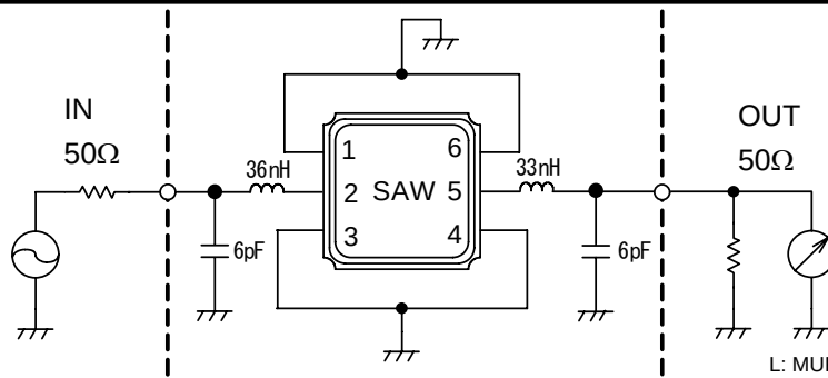
Fig.1 Measuring circuit
