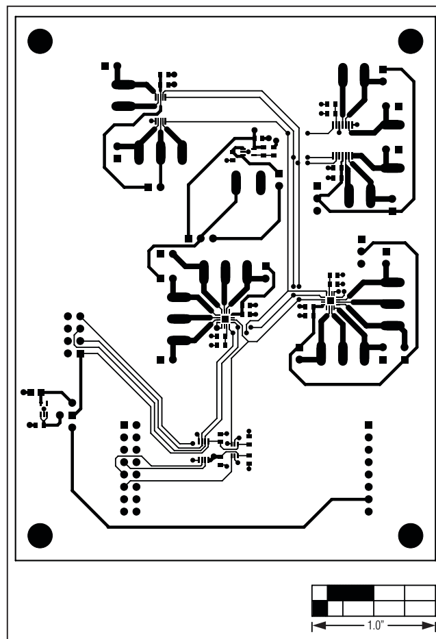
Figure 6. MAX5393 EV Kit PCB Layout—Component Side
