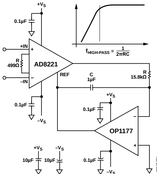
Figure 52. AC-Coupled Circuit
