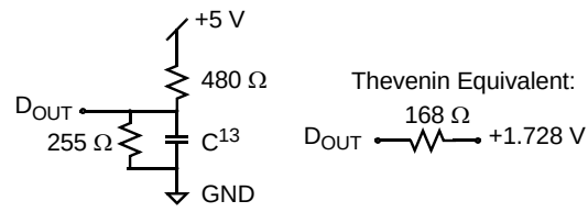
Figure B: 5 V Output load
