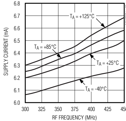
SUPPLY CURRENT vs. RF FREQUENCY (ASK MODE)
