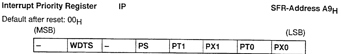
Figure 13 Interrupt Priority Register IP
